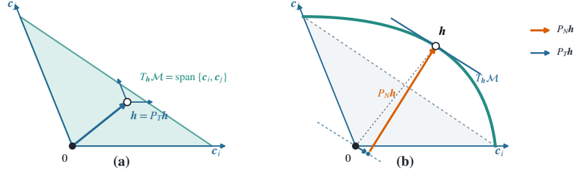
Figure 1: (a) Linearly represented concepts exist on the tangent plane to the manifold. (b) Nonlinear components don't project cleanly onto the tangent space, but incorporate substantial normal data.
