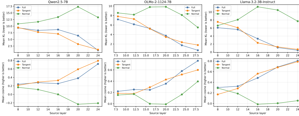
Figure 4: Layerwise average KL divergence (top) and cosine similarity (bottom) between the network output f(\mathbf{h}_\ell) and the three linear approximations we study: \mathbb{E}[J]\mathbf{h}_\ell , \mathbb{E}[J]P_T\mathbf{h}_\ell , and \mathbb{E}[J]P_N\mathbf{h}_\ell .
