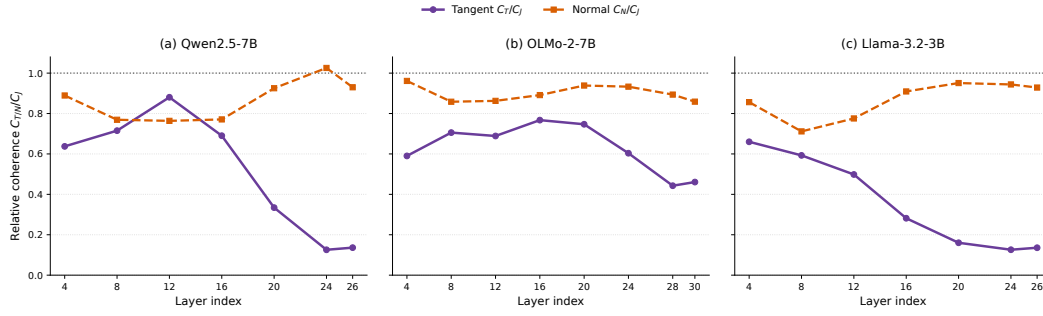
Figure 3: Relative coherence of the tangent and normal projected Jacobians across layers (1=relative coherence of the full Jacobian). As layer index increases, relative coherence of the tangent-projected Jacobian substantially decreases, particularly for Qwen and LLaMA.
