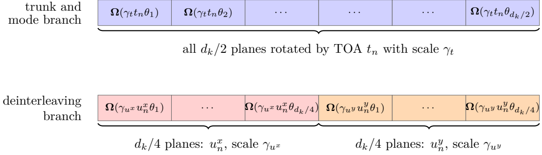
Figure 4.5. Allocation of the d_k/2 rotation planes of one attention head to physical coordinates. In the shared trunk and the mode branch (top), every plane is rotated by the TOA t_n down its frequency ladder (Equation (4.21)); the arrival direction is excluded because the mode embedding should be invariant to viewing geometry. In the deinterleaving branch (bottom), the planes are split evenly into two slices of d_k/4 planes, rotated by u_n^x and u_n^y respectively (Equation (4.24)), so that the attention logit decomposes into the per-coordinate relative terms of Equation (4.25); the TOA is not repeated here because the branch operates on trunk representations that are already TOA-rotated.
