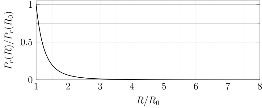
Figure 2.1. Normalized received power versus normalized range from Equation (2.3) with fixed P_t , G , \lambda , and \sigma . Doubling R cuts P_r by a factor of 16.
