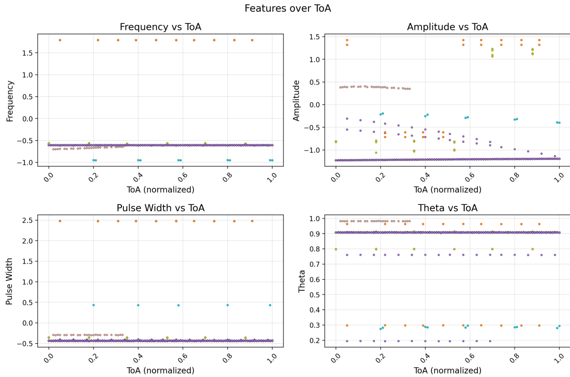
Figure 5.3. A crowded emitter mixture, colored by emitter.
