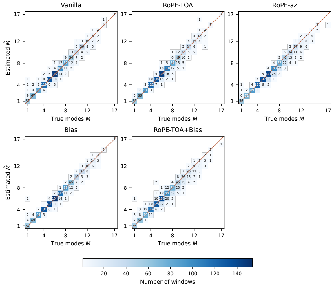
Figure 5.12. Estimated versus true number of modes per test window. Layout as in Figure 5.11.
