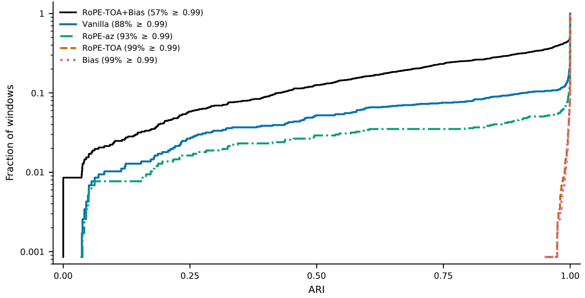
Figure 5.9. Empirical CDF of emitter ARI over the 1168 non-overlapping test windows. The vertical axis is logarithmic.
