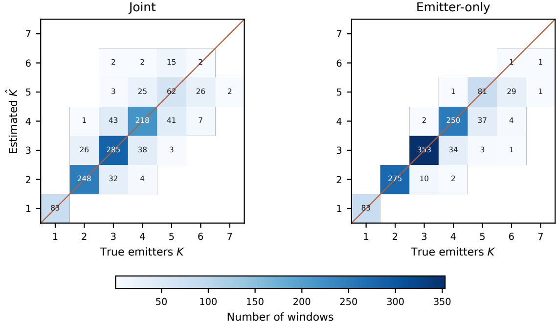
Figure 5.7. Estimated versus true number of emitters per test window for Joint and Emitter-only Vanilla. Cell values are window counts. The line is \hat{K} = K . The Joint panel is the Vanilla evaluation of Table 5.4.
