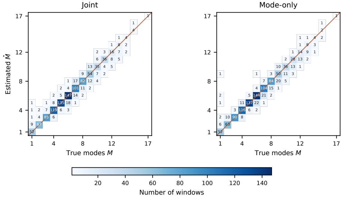
Figure 5.8. Estimated versus true number of modes per test window for Joint and Mode-only Vanilla. Layout as in Figure 5.7.
