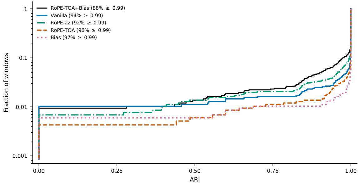
Figure 5.10. Empirical CDF of mode ARI over the same windows as Figure 5.9. The vertical axis is logarithmic.
