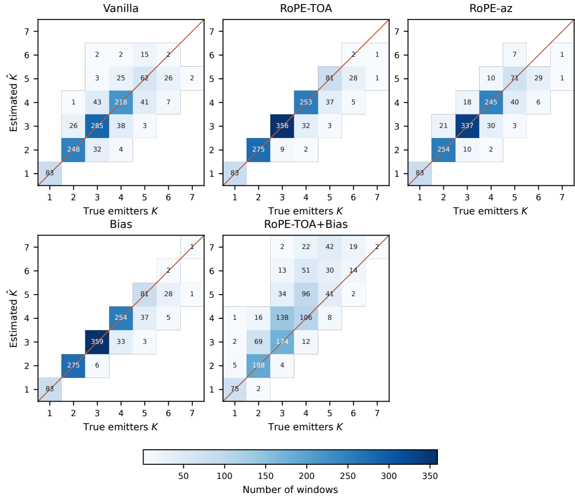
Figure 5.11. Estimated versus true number of emitters per test window. Cell values are window counts. The line is \hat{K} = K .
