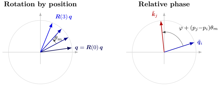
Figure 4.6. Geometry of RoPE on one of the d_k/2 two-dimensional planes of a head. Left: increasing the coordinate p rotates a query vector \mathbf{q} at a fixed rate \theta_m (Equation (4.18)), so the absolute coordinate is encoded as an absolute phase; here p takes the integer values 0, \dots, 3 , but any real coordinate such as the TOA is admissible. Right: the angle enclosed between a rotated query \tilde{\mathbf{q}}_i and a rotated key \tilde{\mathbf{k}}_j equals the content angle plus (p_j - p_i)\theta_m ; since the inner product depends only on this enclosed angle, the attention logit is a function of the coordinate difference p_j - p_i (Equation (4.20)).
