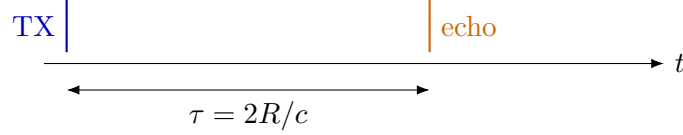
Figure 2.1. Cartoon timeline for one transmit pulse and its monostatic echo; the measured delay maps to range through Equation (2.1).
