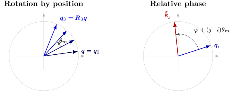
Figure 4.5. Geometry of RoPE on one of the d_k/2 two-dimensional planes of a head. Left: increasing the position index i rotates a query vector q by a fixed increment \theta_m per step (Equation (4.18)), so absolute position is encoded as an absolute phase. Right: the angle enclosed between a rotated query \tilde{q}_i and a rotated key \tilde{k}_j equals the content angle plus (j-i)\theta_m ; since the inner product depends only on this enclosed angle, the attention logit is a function of the relative position j-i (Equation (4.19)).
