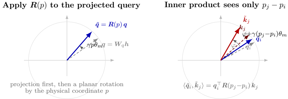
Figure 4.6. Geometry of RoPE on one of the d_k/2 two-dimensional planes of a head. Left: the projected query q = W_q h (dashed) is obtained exactly as in vanilla attention (Equation (4.17)); RoPE then applies the planar rotation R(p) of Equation (4.21), adding a modest absolute phase \gamma p \theta_m . Right: after both the query and the key are rotated, the enclosed angle equals the content angle \varphi (dashed pair) plus the relative phase \gamma(p_j - p_i)\theta_m ; the inner product therefore depends on the coordinate difference alone (Equation (4.23)).
