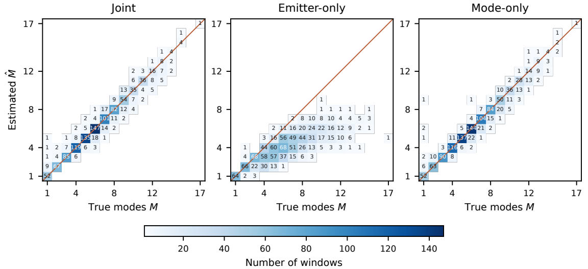
Figure 5.4. Estimated versus true number of modes per test window. Layout as in Figure 5.3.
