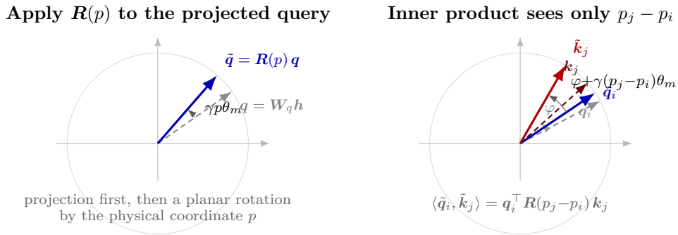
Figure 4.6. Geometry of RoPE on one of the d_k/2 two-dimensional planes of a head. Left: the projected query \mathbf{q} = \mathbf{W}_q \mathbf{h} (dashed) is obtained exactly as in vanilla attention (Equation (4.17)); RoPE then applies the planar rotation \mathbf{R}(p) of Equation (4.21), adding a modest absolute phase \gamma p \theta_m . Right: after both the query and the key are rotated, the enclosed angle equals the content angle \varphi (dashed pair) plus the relative phase \gamma(p_j - p_i)\theta_m ; the inner product therefore depends on the coordinate difference alone (Equation (4.23)).
