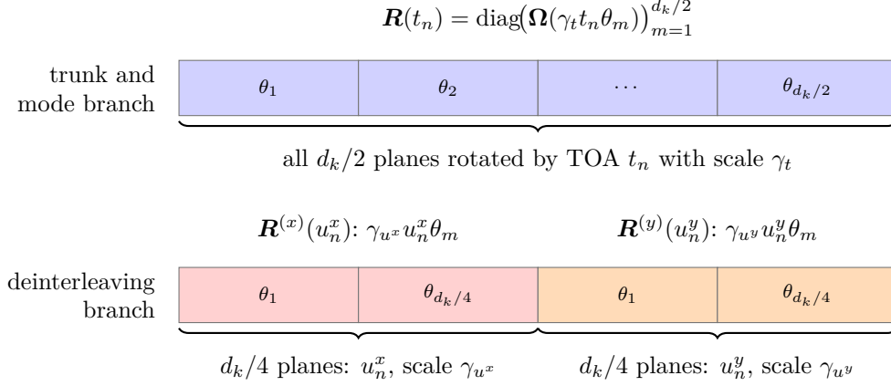
Figure 4.5. Allocation of the d_k/2 rotation planes of one attention head to physical coordinates. Each strip is headed by the rotation that is applied and the corresponding scale \gamma ; the cells list the per-plane frequencies \theta_m of Equation (4.21). In the shared trunk and the mode branch (top), every plane is rotated by the TOA t_n with scale \gamma_t ; the arrival direction is excluded because the mode embedding should be invariant to viewing geometry. In the deinterleaving branch (bottom), the planes are split evenly into two slices of d_k/4 planes, rotated by u_n^x and u_n^y with scales \gamma_{u^x} and \gamma_{u^y} respectively (Equation (4.24)), so that the attention logit decomposes into the per-coordinate relative terms of Equation (4.25); the TOA is not repeated here because the branch operates on trunk representations that are already TOA-rotated.
