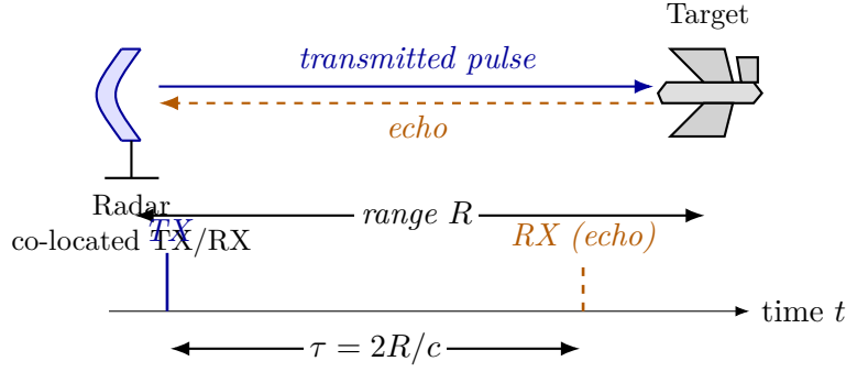
Figure 2.1. Monostatic radar geometry and round-trip timing. A co-located transmit/receive (TX/RX) aperture on the left emits a pulse that travels to a target at range R , scatters, and returns to the same aperture as an echo. The lower timeline shows the corresponding events: the outgoing TX pulse at t = 0 and the received echo at t = \tau , separated by the round-trip delay \tau = 2R/c from Equation (2.1).
