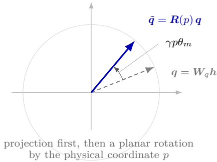
Apply R(p) to the projected query
