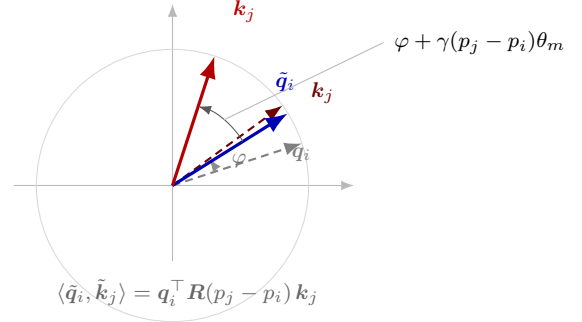
Inner product sees only p_j - p_i
