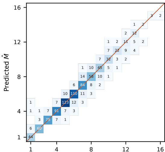
RoPE-az
