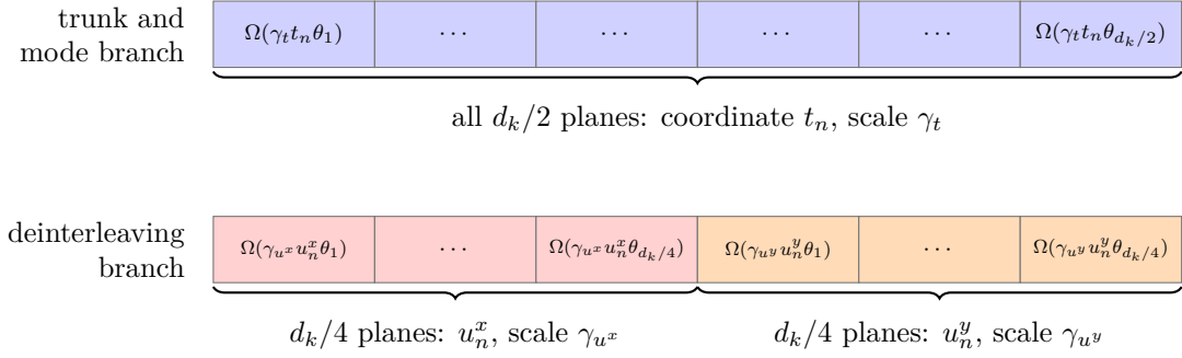
Figure 4.5. Allocation of the d_k/2 rotation planes of one attention head to physical coordinates. In the shared trunk and the mode branch (top), every plane is rotated by the TOA t_n with scale \gamma_t (Equation (4.21)); the arrival direction is excluded because the mode embedding should be invariant to viewing geometry. In the deinterleaving branch (bottom), the planes are split evenly into two slices of d_k/4 planes, rotated by u_n^x and u_n^y with scales \gamma_{u^x} and \gamma_{u^y} respectively (Equation (4.24)), so that the attention logit decomposes into the per-coordinate relative terms of Equation (4.25); the TOA is not repeated here because the branch operates on trunk representations that are already TOA-rotated. Ellipsis cells indicate the intermediate planes of each frequency ladder.
