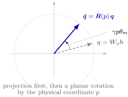
Figure 4.6. Geometry of RoPE on one of the d_k/2 two-dimensional planes of a head. Left: the projected query \mathbf{q} = \mathbf{W}_q \mathbf{h} (dashed) is obtained exactly as in vanilla attention (Equation (4.17)); RoPE then applies the planar rotation \mathbf{R}(p) of Equation (4.21), adding a modest absolute phase \gamma p \theta_m . Right: after both the query and the key are rotated, the enclosed angle equals the content angle \varphi (dashed pair) plus the relative phase \gamma(p_j - p_i)\theta_m ; the inner product therefore depends on the coordinate difference alone (Equation (4.23)).
