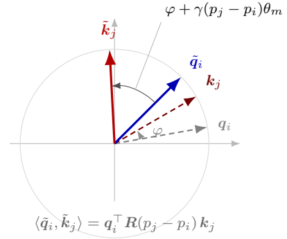
Figure 4.6. Geometry of RoPE on one of the d_k/2 two-dimensional planes of a head. Left: the projected query \mathbf{q} = \mathbf{W}_q \mathbf{h} (dashed) is obtained exactly as in vanilla attention (Equation (4.17)); RoPE then applies the planar rotation \mathbf{R}(p) of Equation (4.21), adding a modest absolute phase \gamma p \theta_m . Right: after both the query and the key are rotated, the enclosed angle equals the content angle \varphi (dashed pair) plus the relative phase \gamma(p_j - p_i)\theta_m ; the inner product therefore depends on the coordinate difference alone (Equation (4.23)).
