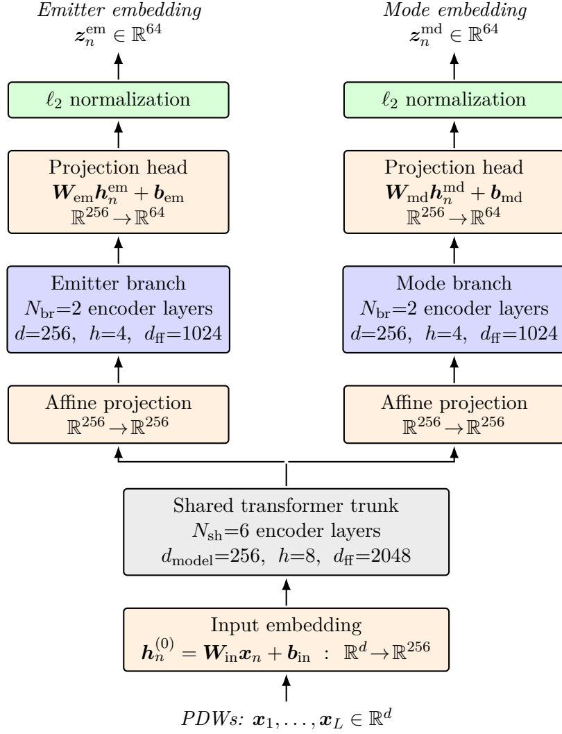
Figure 4.3. Architecture of the encoder f_{\theta} . A sequence of PDWs is first lifted to d_{model} = 256 by an affine input embedding, processed by a shared trunk of 6 transformer-encoder layers, and then split into two parallel branches, each with its own affine 256 \rightarrow 256 projection and 2 encoder layers. Branch outputs are mapped by affine projection heads to the 64-dimensional emitter and mode embedding spaces and \ell_2 -normalized over the embedding dimension. The input embedding, branch projections, and projection heads are all affine maps of the same form.
