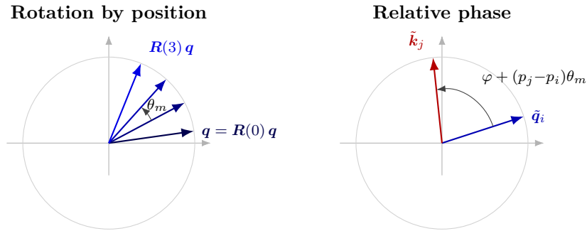
Figure 4.6. Geometry of RoPE on one of the d_k/2 two-dimensional planes of a head. Left: increasing the coordinate p rotates a query vector \mathbf{q} at a fixed rate \gamma\theta_m (Equation (4.21)), so the absolute coordinate is encoded as an absolute phase; here p takes the integer values 0, \dots, 3 , but any real coordinate such as the TOA is admissible. Right: the angle enclosed between a rotated query \tilde{\mathbf{q}}_i and a rotated key \tilde{\mathbf{k}}_j equals the content angle plus \gamma(p_j - p_i)\theta_m ; since the inner product depends only on this enclosed angle, the attention logit is a function of the coordinate difference p_j - p_i (Equation (4.23)).
