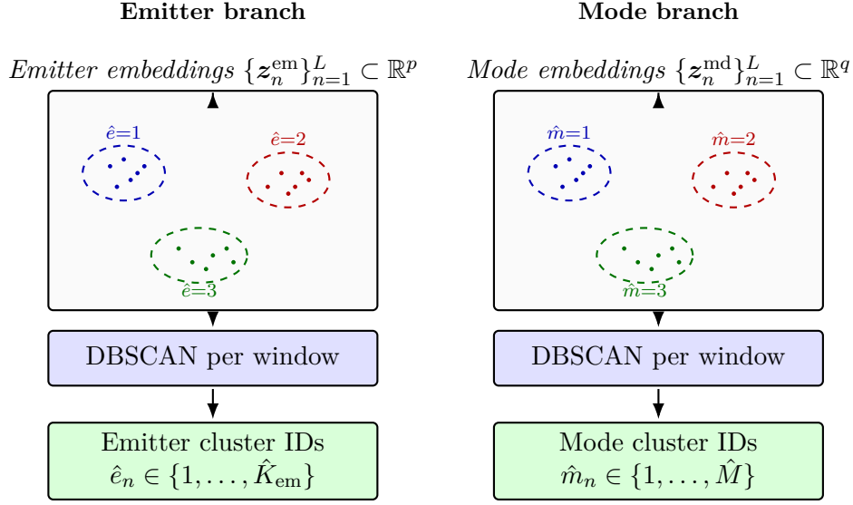
Figure 4.4. Inference-time decoding of branch embeddings into per-pulse cluster indices via Equation (4.18). Dots are pulse embeddings and dashed ellipses are DBSCAN clusters in one window. The pipeline is identical on both branches and the integer outputs are local to each clustering instance; they acquire their interpretation from the supervision scope of Section 4.1, which differs between the two branches.
