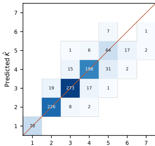
RoPE-az
