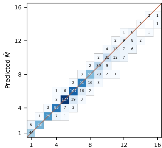
True modes M
