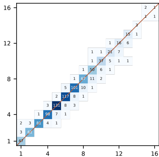
True modes M
