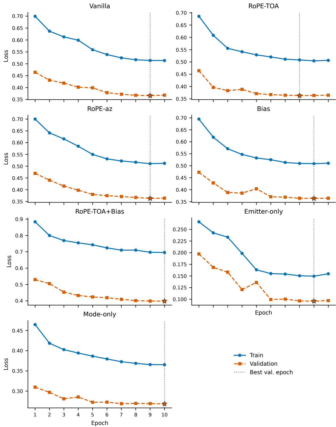
Figure 5.4. Training and validation loss versus epoch. The star and dotted line mark the epoch of lowest validation loss.
