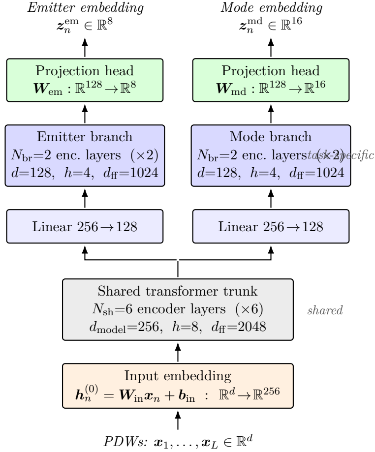
Figure 4.2. Architecture of the encoder f_\theta . A sequence of PDWs is first lifted to d_{model} = 256 by an input embedding, processed by a shared trunk of 6 transformer-encoder layers, and then split into two parallel branches with their own 256 \rightarrow 128 projection and 2 encoder layers. Branch outputs are mapped by linear projection heads to the emitter embedding space \mathbb{R}^8 and the mode embedding space \mathbb{R}^{16} .
