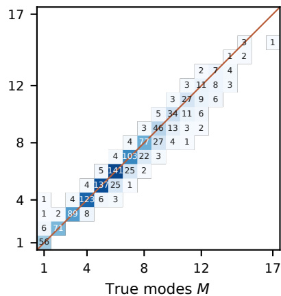
RoPE-az
