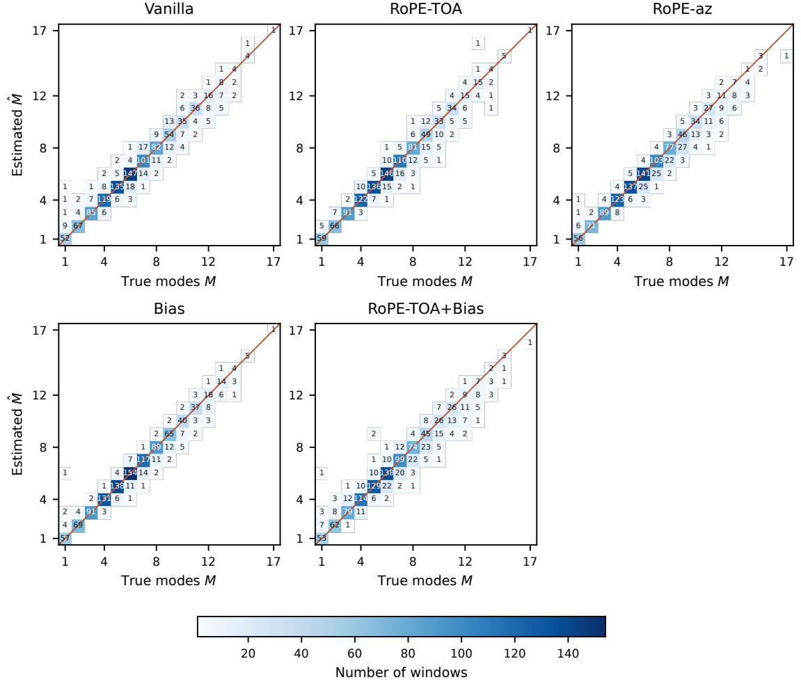
Figure 5.8. Predicted versus true number of modes per test window. Layout as in Figure 5.7.
