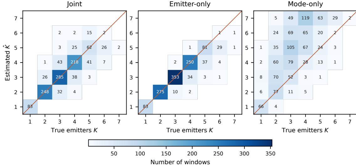
Figure 5.3. Predicted versus true number of emitters per test window for the three Vanilla objectives. Cell values are window counts. The line is \hat{K} = K . The Joint panel is the Vanilla evaluation of Table 5.4.
