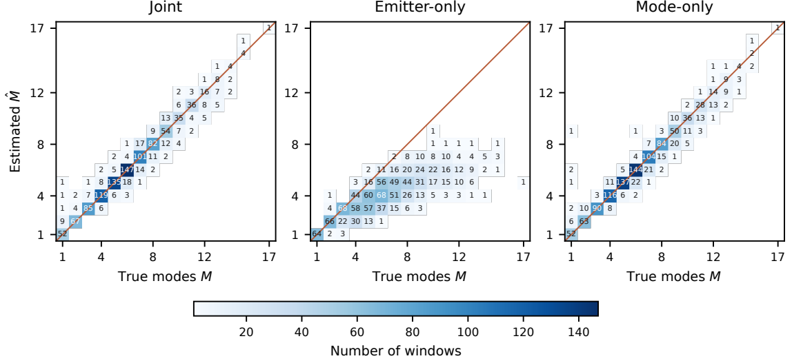
Figure 5.4. Predicted versus true number of modes per test window. Layout as in Figure 5.3.
