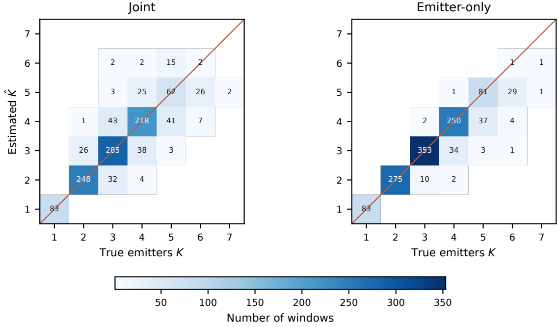
Figure 5.3. Estimated versus true number of emitters per test window for Joint and Emitter-only Vanilla. Cell values are window counts. The line is \hat{K} = K . The Joint panel is the Vanilla evaluation of Table 5.4.
