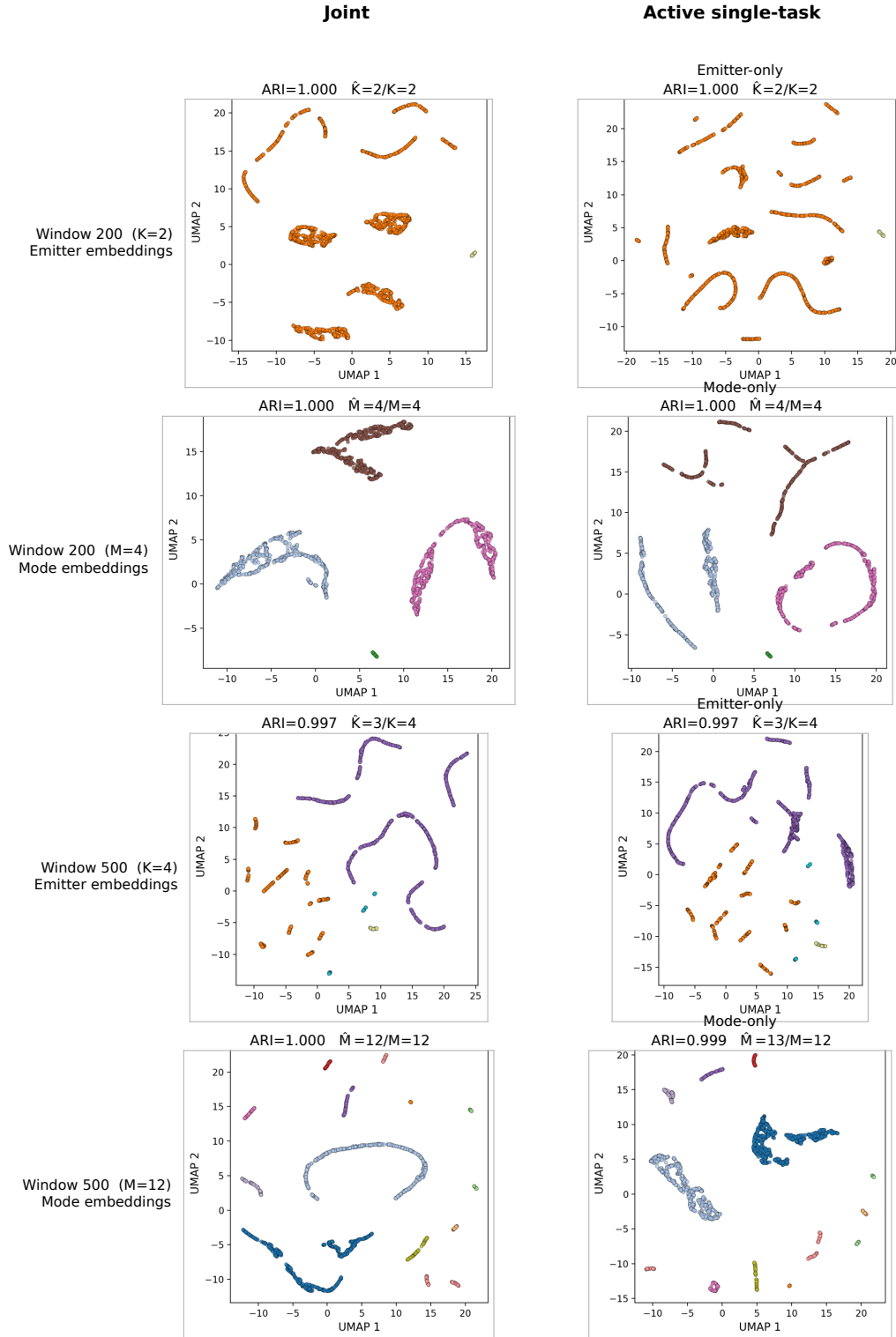
Figure 5.2. UMAP of active-branch embeddings on two test windows, colored by ground-truth labels. Columns are Joint and the matching single-task run. Rows alternate emitter and mode embeddings. Window 200 has K = 2 and M = 4 ; window 500 has K = 4 and M = 12 .
