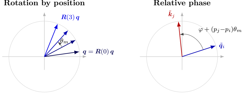
Figure 4.5. Geometry of RoPE on one of the d_k/2 two-dimensional planes of a head. Left: increasing the coordinate p rotates a query vector \mathbf{q} at a fixed rate \theta_m (Equation (4.17)), so the absolute coordinate is encoded as an absolute phase; here p takes the integer values 0, \dots, 3 , but any real coordinate such as the TOA is admissible. Right: the angle enclosed between a rotated query \tilde{\mathbf{q}}_i and a rotated key \tilde{\mathbf{k}}_j equals the content angle plus (p_j - p_i)\theta_m ; since the inner product depends only on this enclosed angle, the attention logit is a function of the coordinate difference p_j - p_i (Equation (4.18)).
