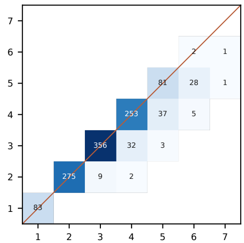
Bias
