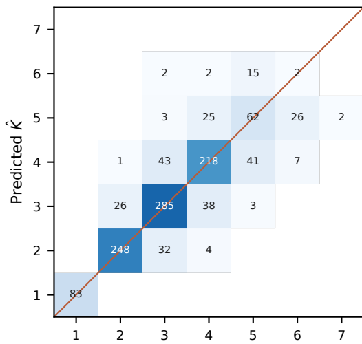
RoPE-az
