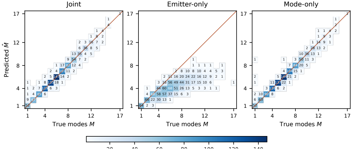
Figure 5.4. Predicted versus true number of modes per test window. Layout as in Figure 5.3.
