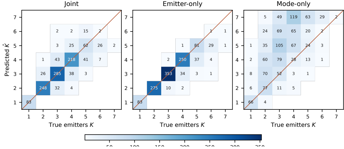
Figure 5.3. Predicted versus true number of emitters per test window for the three Vanilla objectives. Cell values are window counts. The line is \hat{K} = K . The Joint panel is the Vanilla evaluation of Table 5.4.
