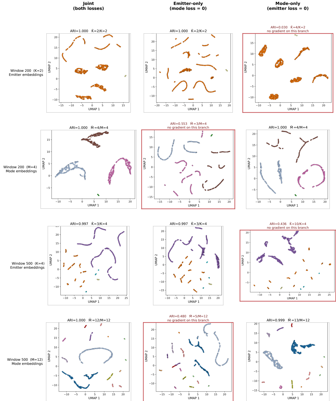
Figure 5.2. UMAP of Vanilla embeddings on two test windows, coloured by ground-truth labels. Columns are Joint, Emitter-only, and Mode-only. Rows alternate emitter and mode branches. Red frames mark the unused branch. Window 200 is test scenario 1793 ( K = 2 , M = 4 ); window 500 is scenario 1858 ( K = 4 , M = 12 ).
