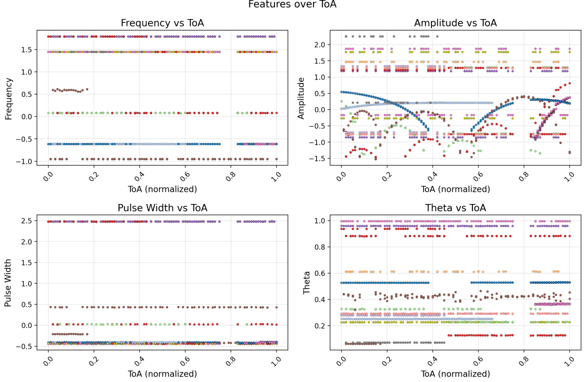
Figure 5.4. A crowded mode mixture, colored by ground-truth mode.
