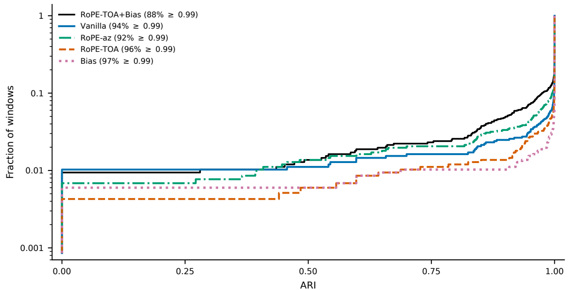
Figure 5.6. Empirical CDF of mode ARI over the same windows as Figure 5.5. The vertical axis is logarithmic.
