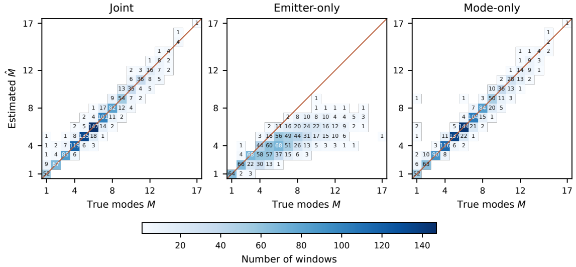
Figure 5.4. Estimated versus true number of modes per test window. Layout as in Figure 5.3.
