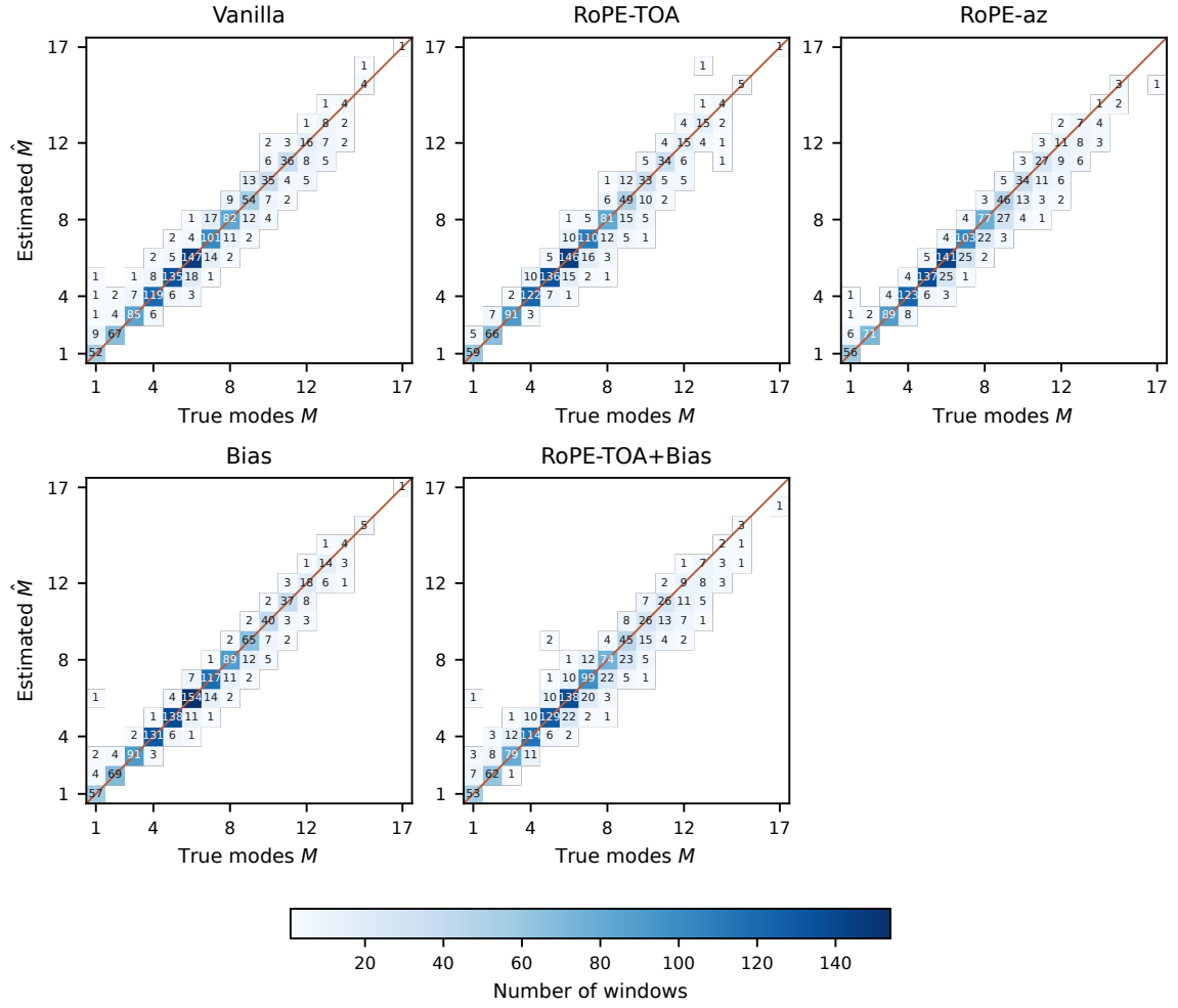
Figure 5.8. Estimated versus true number of modes per test window. Layout as in Figure 5.7.
