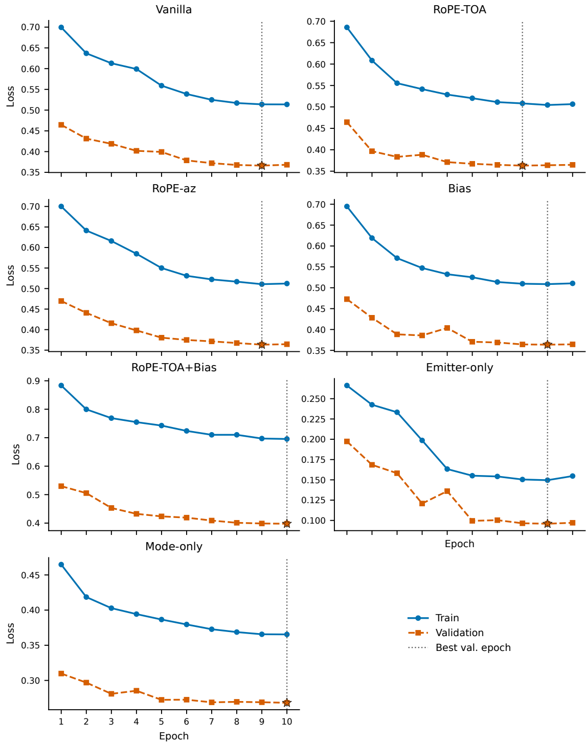
Figure 5.1. Training and validation loss versus epoch. The star and dotted line mark the epoch of lowest validation loss.
