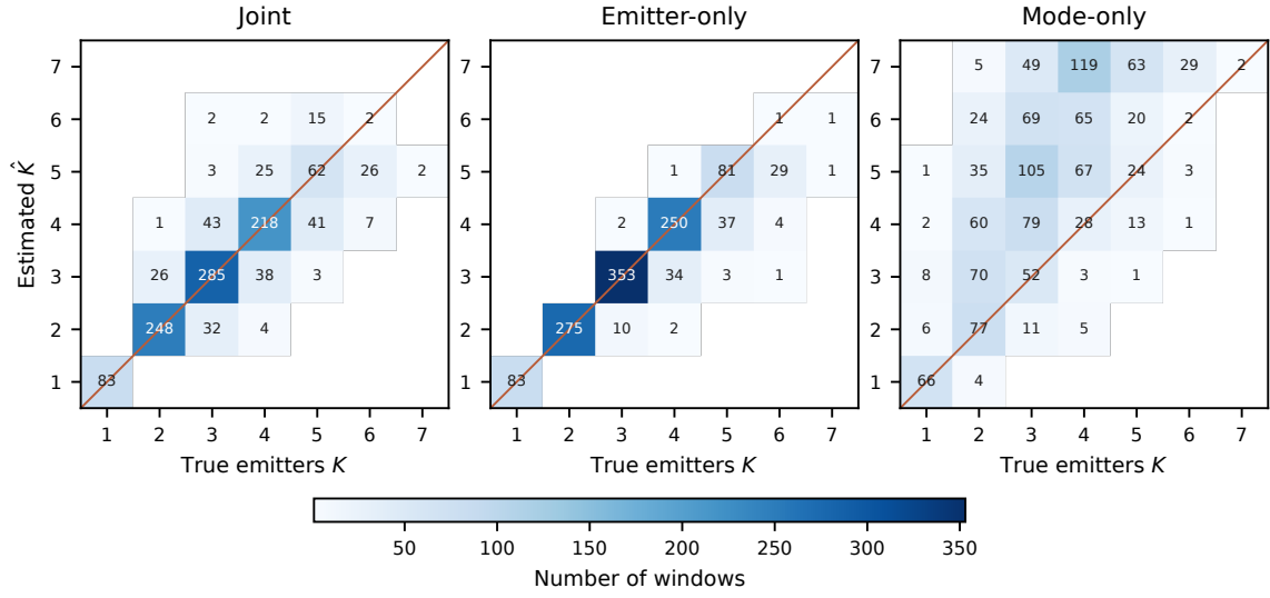
Figure 5.3. Estimated versus true number of emitters per test window for the three Vanilla objectives. Cell values are window counts. The line is \hat{K} = K . The Joint panel is the Vanilla evaluation of Table 5.4.
