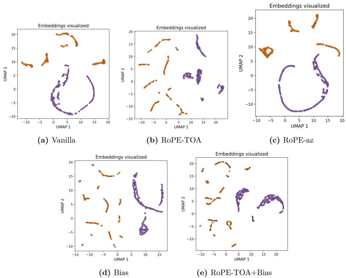
Figure 5.12. UMAP of emitter-branch embeddings on test scenario 1752, colored by ground-truth emitter.
