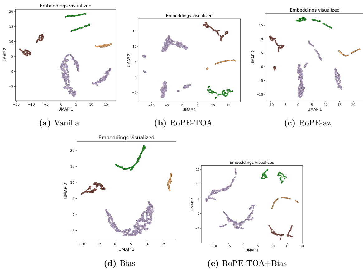
Figure 5.13. UMAP of mode-branch embeddings on test scenario 1752, colored by ground-truth mode.
