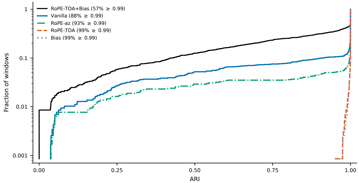
Figure 5.5. Empirical CDF of emitter ARI over the 1168 non-overlapping test windows. The vertical axis is logarithmic.
