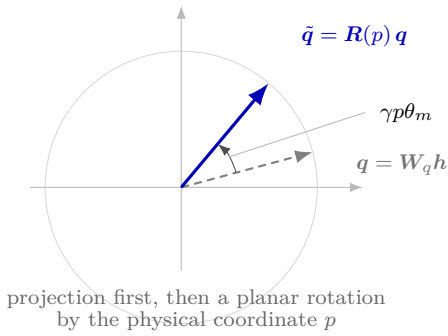
Figure 4.6. Geometry of RoPE on one of the d_k/2 two-dimensional planes of a head. Left: the projected query \mathbf{q} = \mathbf{W}_q \mathbf{h} (dashed) is obtained exactly as in vanilla attention (Equation (4.17)); RoPE then applies the planar rotation \mathbf{R}(p) of Equation (4.21), adding a modest absolute phase \gamma p \theta_m . Right: after both the query and the key are rotated, the enclosed angle equals the content angle \varphi (dashed pair) plus the relative phase \gamma(p_j - p_i)\theta_m ; the inner product therefore depends on the coordinate difference alone (Equation (4.23)).
