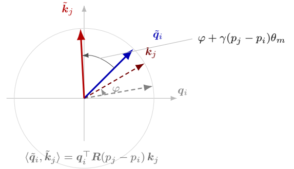
Figure 4.6. Geometry of RoPE on one of the d_k/2 two-dimensional planes of a head. Left: the projected query \mathbf{q} = \mathbf{W}_q \mathbf{h} (dashed) is obtained exactly as in vanilla attention (Equation (4.17)); RoPE then applies the planar rotation \mathbf{R}(p) of Equation (4.21), adding a modest absolute phase \gamma p \theta_m . Right: after both the query and the key are rotated, the enclosed angle equals the content angle \varphi (dashed pair) plus the relative phase \gamma(p_j - p_i)\theta_m ; the inner product therefore depends on the coordinate difference alone (Equation (4.23)).
