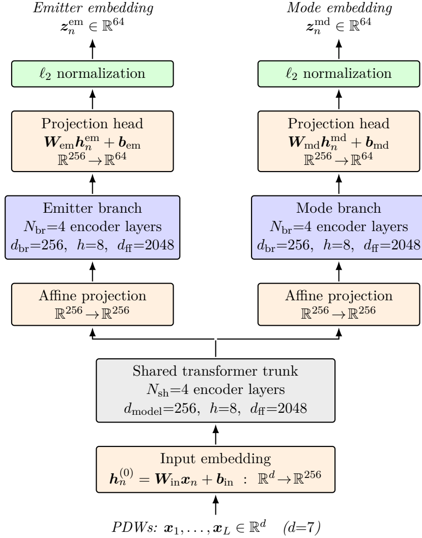
Figure 4.3. Architecture of the encoder f_\theta . Each pulse is the d = 7 -dimensional scaled PDW of Section 4.2. A sequence of such vectors is first lifted to d_{model} = 256 by an affine input embedding, processed by a shared trunk of 4 transformer-encoder layers, and then split into two parallel branches, each with its own affine 256 \rightarrow 256 projection and 4 encoder layers. Branch outputs are mapped by affine projection heads to the 64-dimensional emitter and mode embedding spaces and \ell_2 -normalized over the embedding dimension. The input embedding, branch projections, and projection heads are all affine maps of the same form.
