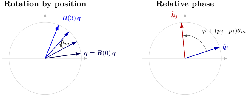
Figure 4.6. Geometry of RoPE on one of the d_k/2 two-dimensional planes of a head. Left: increasing the coordinate p rotates a query vector \mathbf{q} at a fixed rate \theta_m (Equation (4.22)), so the absolute coordinate is encoded as an absolute phase; here p takes the integer values 0, \dots, 3 , but any real coordinate such as the TOA is admissible. Right: the angle enclosed between a rotated query \tilde{\mathbf{q}}_i and a rotated key \tilde{\mathbf{k}}_j equals the content angle plus (p_j - p_i)\theta_m ; since the inner product depends only on this enclosed angle, the attention logit is a function of the coordinate difference p_j - p_i (Equation (4.24)).
