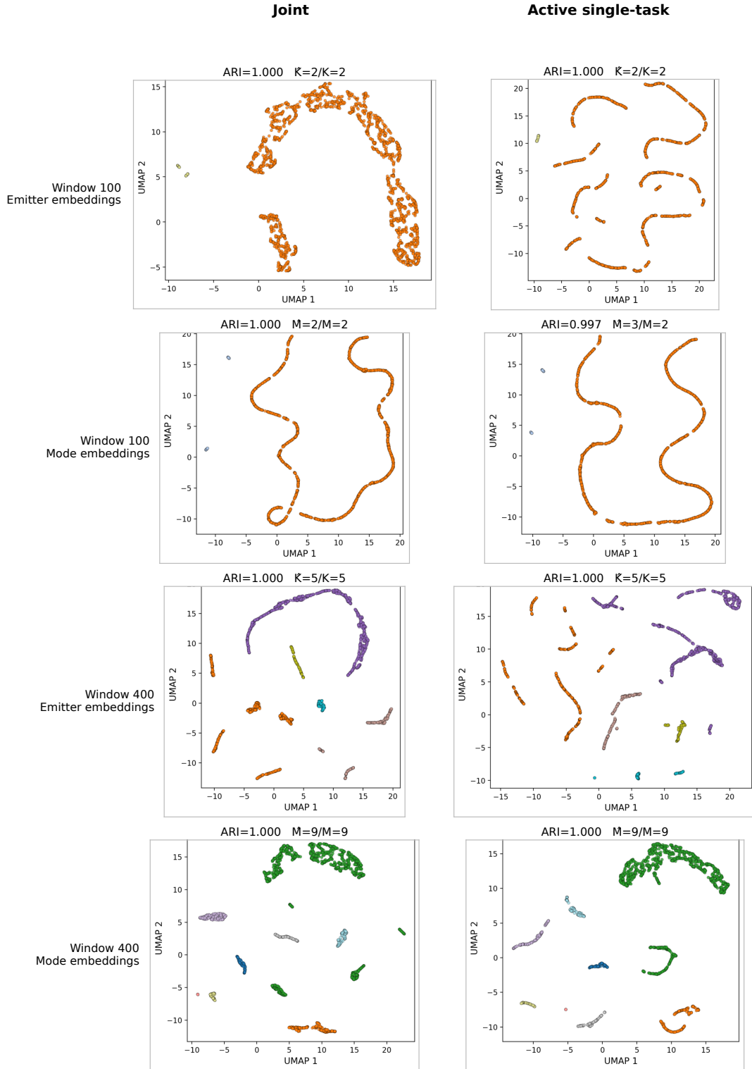
Figure 5.6. UMAP of active-branch embeddings on two test windows, colored by ground-truth labels. Columns are Joint and the matching single-task run. Rows alternate emitter and mode embeddings. Window 100 has K = 2 and M = 2 ; window 400 has K = 5 and M = 9 .
