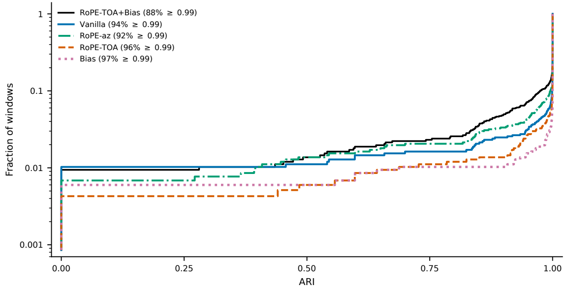
Figure 5.10. Empirical CDF of mode ARI over the same windows as Figure 5.9. The vertical axis is logarithmic.
