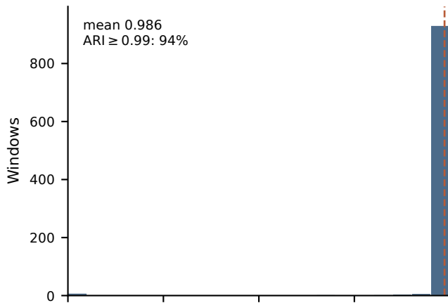
RoPE-az
