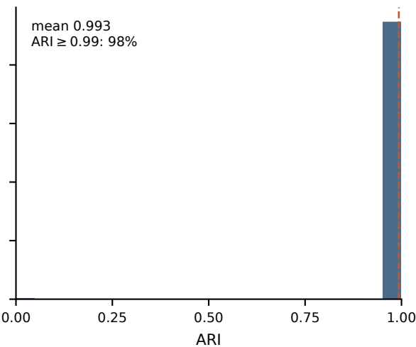
Bias
