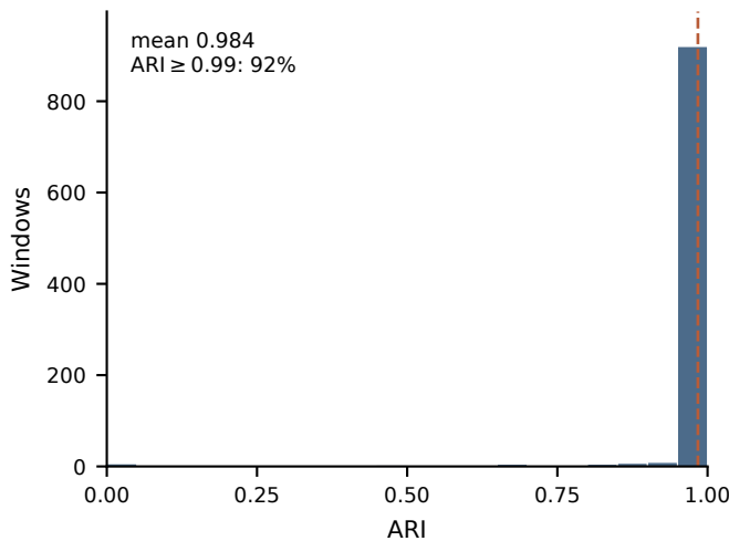
RoPE-az
