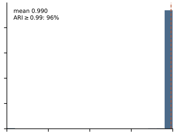
Bias
