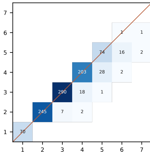
Bias
