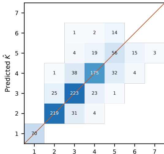
RoPE-az
