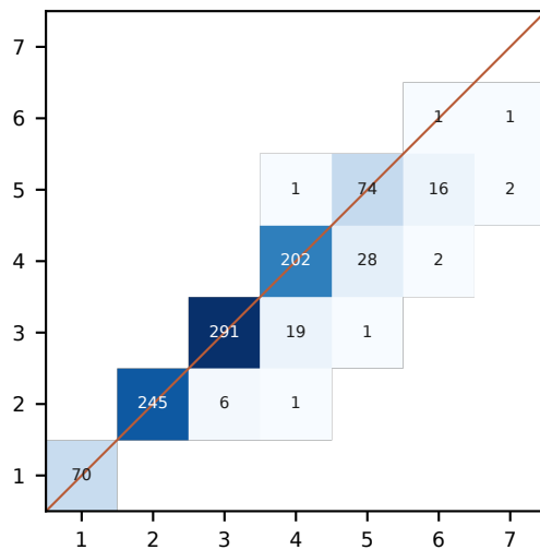
Bias
