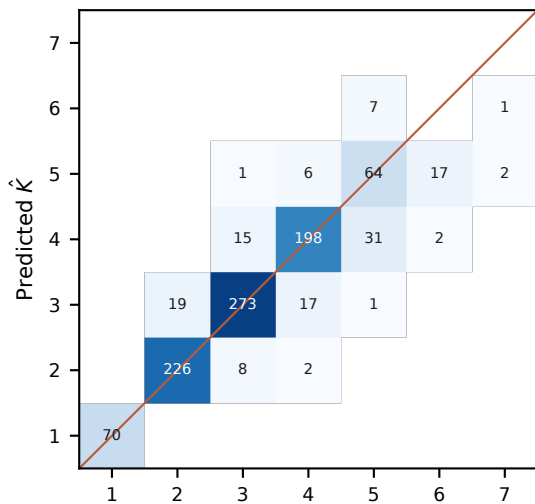
RoPE-az
