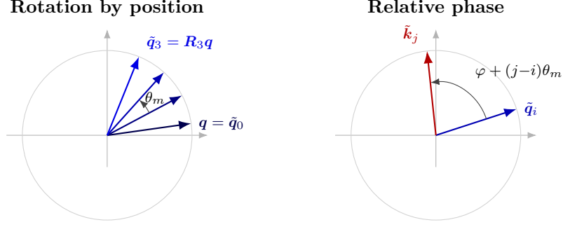
Figure 4.5. Geometry of RoPE on one of the d_k/2 two-dimensional planes of a head. Left: increasing the position index i rotates a query vector \mathbf{q} by a fixed increment \theta_m per step (Equation (4.18)), so absolute position is encoded as an absolute phase. Right: the angle enclosed between a rotated query \tilde{\mathbf{q}}_i and a rotated key \tilde{\mathbf{k}}_j equals the content angle plus (j-i)\theta_m ; since the inner product depends only on this enclosed angle, the attention logit is a function of the relative position j-i (Equation (4.19)).
