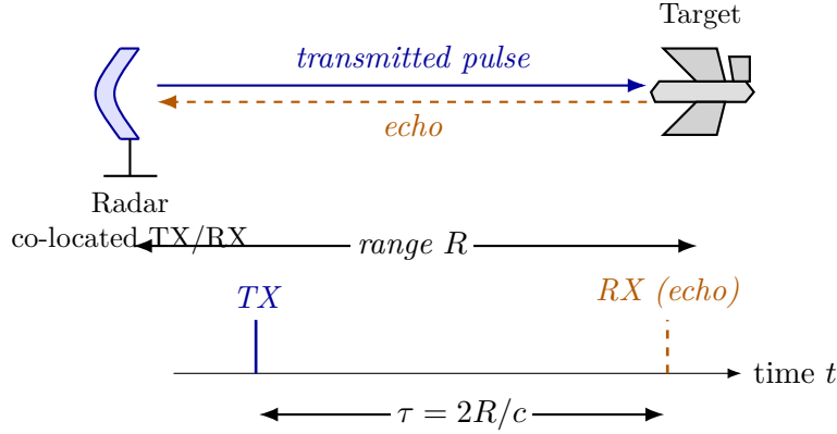
Figure 2.1. Monostatic radar geometry and round-trip timing. A co-located transmit/receive (TX/RX) aperture on the left emits a pulse that travels to a target at range R , scatters, and returns to the same aperture as an echo. The lower timeline shows the corresponding events: the outgoing TX pulse at t = 0 and the received echo at t = \tau , separated by the round-trip delay \tau = 2R/c from Equation (2.1).
