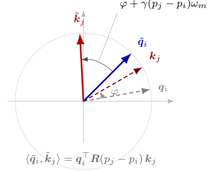
Figure 4.5. Geometry of RoPE on one of the d_k/2 two-dimensional planes of a head. Left: the projected query q = W_q h (dashed) is obtained exactly as in vanilla attention (Equation (4.19)); RoPE then applies the planar rotation R(p) of Equation (4.23), adding a modest absolute phase \gamma p \omega_m . Right: after both the query and the key are rotated, the enclosed angle equals the content angle \varphi (dashed pair) plus the relative phase \gamma(p_j - p_i)\omega_m ; the inner product therefore depends on the coordinate difference alone (Equation (4.25)).
