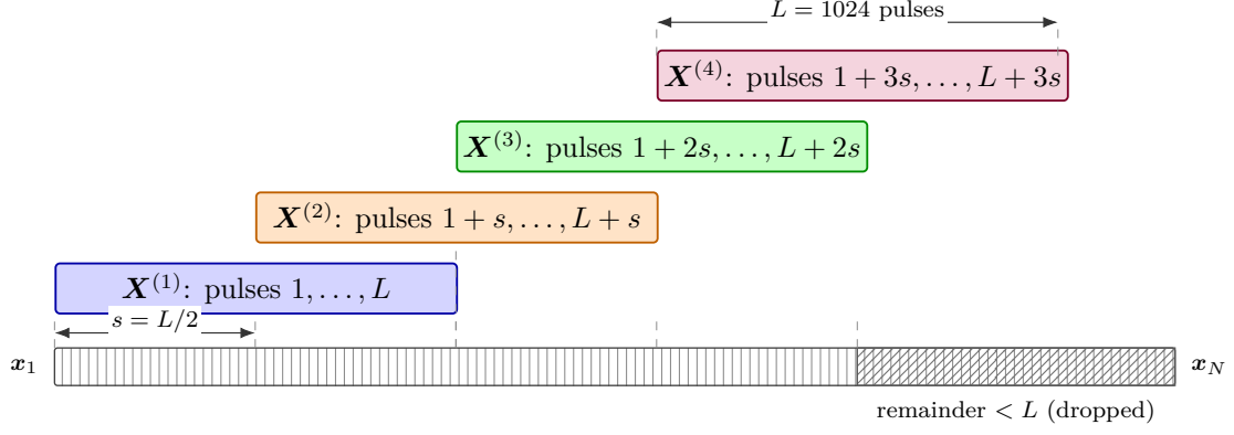
Figure 4.2. Sliding-window segmentation of a pulse train as defined in Equation (4.6), drawn for the training-time stride s = L/2 . Successive windows \mathbf{X}^{(w)} advance by s pulses, so they overlap by L - s = L/2 . Dashed guides project window boundaries down onto the pulse train. Pulses past the last window of length L form a trailing remainder that is dropped during training and evaluation. Validation and test use s = L , giving abutting non-overlapping windows; the dropped remainder remains shorter than L by construction.
