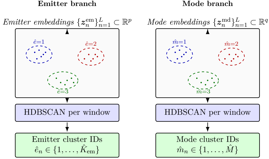
Figure 4.4. Inference-time decoding of branch embeddings into per-pulse cluster indices via Equation (4.14). Dots are pulse embeddings and dashed ellipses are HDBSCAN clusters in one window. The pipeline is identical on both branches and the integer outputs are local to each clustering instance; they acquire their interpretation from the supervision scope of Section 4.1, which differs between the two branches.
