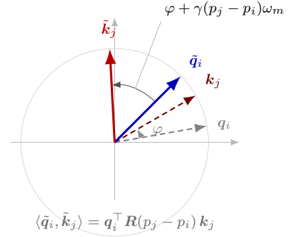
Figure 4.6. Geometry of RoPE on one of the d_k/2 two-dimensional planes of a head. Left : the projected query q = W_q h (dashed) is obtained exactly as in vanilla attention (Equation (4.18)); RoPE then applies the planar rotation R(p) of Equation (4.22), adding a modest absolute phase \gamma p \omega_m . Right : after both the query and the key are rotated, the enclosed angle equals the content angle \varphi (dashed pair) plus the relative phase \gamma(p_j - p_i)\omega_m ; the inner product therefore depends on the coordinate difference alone (Equation (4.24)).
