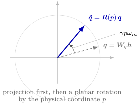
Figure 4.6. Geometry of RoPE on one of the d_k/2 two-dimensional planes of a head. Left : the projected query q = W_q h (dashed) is obtained exactly as in vanilla attention (Equation (4.18)); RoPE then applies the planar rotation R(p) of Equation (4.22), adding a modest absolute phase \gamma p \omega_m . Right : after both the query and the key are rotated, the enclosed angle equals the content angle \varphi (dashed pair) plus the relative phase \gamma(p_j - p_i)\omega_m ; the inner product therefore depends on the coordinate difference alone (Equation (4.24)).
