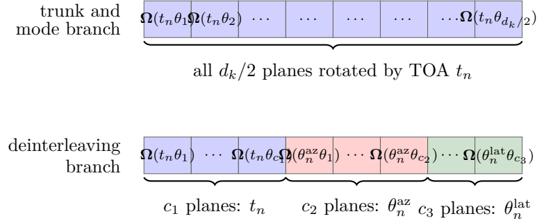
Figure 4.5. Allocation of the d_k/2 rotation planes of one attention head to physical coordinates. In the shared trunk and the mode branch (top), every plane is rotated by the TOA t_n down its frequency ladder (Equation (4.23)); the AOA is excluded because the mode embedding should be invariant to viewing geometry. In the deinterleaving branch (bottom), the planes are partitioned into three disjoint slices of sizes c_1 , c_2 , and c_3 , rotated by t_n , \theta_n^{az} , and \theta_n^{lat} respectively (Equation (4.26)), so that the attention logit decomposes into the per-coordinate relative terms of Equation (4.27).
