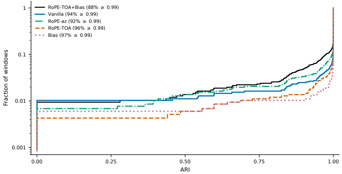
Figure 5.6. Empirical CDF of mode ARI over the same windows as Figure 5.5. The vertical axis is logarithmic.
