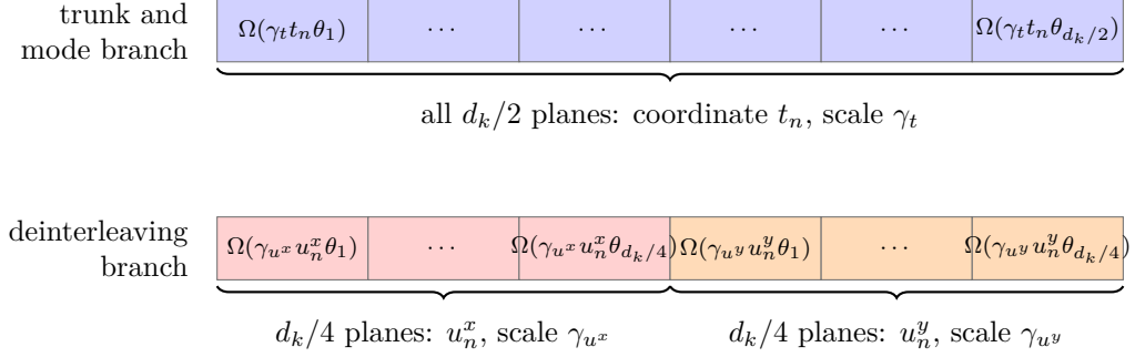
Figure 4.5. Allocation of the d_k/2 rotation planes of one attention head to physical coordinates. In the shared trunk and the mode branch (top), every plane is rotated by the TOA t_n with scale \gamma_t (Equation (4.21)); the arrival direction is excluded because the mode embedding should be invariant to viewing geometry. In the deinterleaving branch (bottom), the planes are split evenly into two slices of d_k/4 planes, rotated by u_n^x and u_n^y with scales \gamma_{u^x} and \gamma_{u^y} respectively (Equation (4.24)), so that the attention logit decomposes into the per-coordinate relative terms of Equation (4.25); the TOA is not repeated here because the branch operates on trunk representations that are already TOA-rotated. Ellipsis cells indicate the intermediate planes of each frequency ladder.
