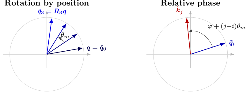
Figure 4.5. Geometry of RoPE on one of the d_k/2 two-dimensional planes of a head. Left: increasing the position index i rotates a query vector \mathbf{q} by a fixed increment \theta_m per step (Equation (4.18)), so absolute position is encoded as an absolute phase. Right: the angle enclosed between a rotated query \tilde{\mathbf{q}}_i and a rotated key \tilde{\mathbf{k}}_j equals the content angle plus (j - i)\theta_m ; since the inner product depends only on this enclosed angle, the attention logit is a function of the relative position j - i (Equation (4.19)).
