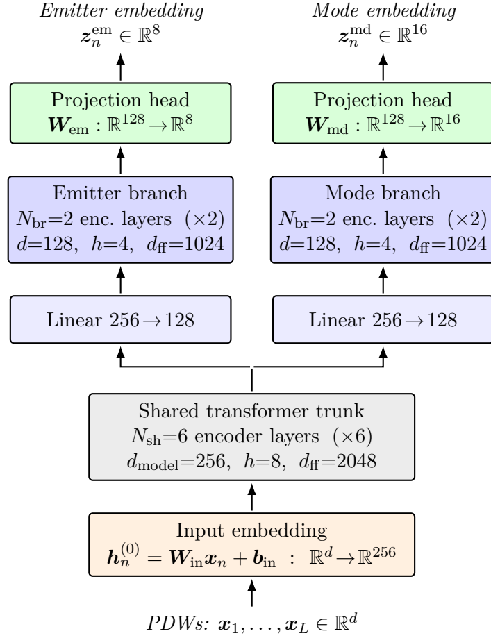
Figure 4.1. Architecture of the encoder f_\theta . A sequence of PDWs is first lifted to d_{\text{model}} = 256 by an input embedding, processed by a shared trunk of 6 transformer-encoder layers, and then split into two parallel branches with their own 256 \rightarrow 128 projection and 2 encoder layers. Branch outputs are mapped by linear projection heads to the emitter embedding space \mathbb{R}^8 and the mode embedding space \mathbb{R}^{16} .
