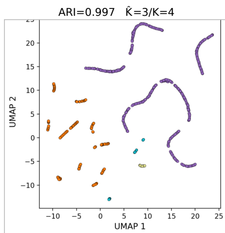
Window 500 (K=4) Emitter embeddings
