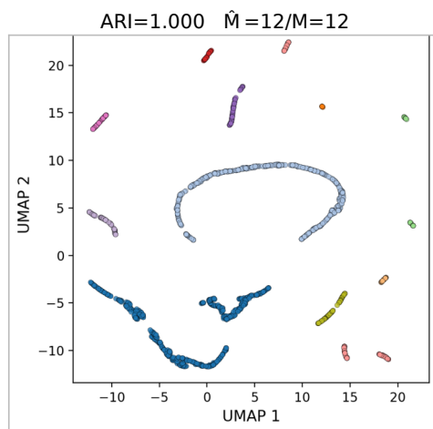
Window 500 (M=12) Mode embeddings
