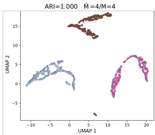
Window 200 (M=4) Mode embeddings
