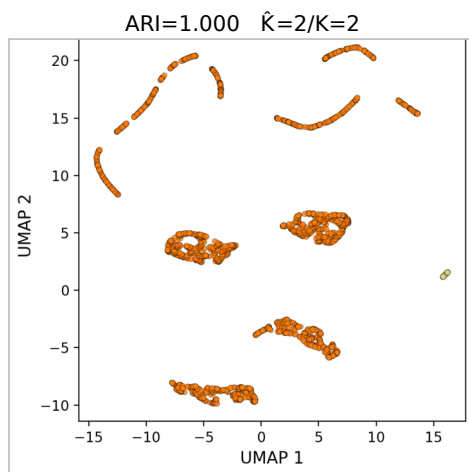
Window 200 (K=2) Emitter embeddings
