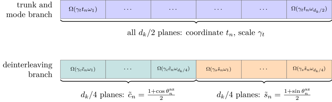
Figure 4.5. Allocation of the d_k/2 rotation planes of one attention head. Top : shared trunk and mode branch—all planes rotated by the TOA t_n with scale \gamma_t (Equation (4.25)). Bottom : deinterleaving branch—planes split evenly between the wrap-safe features \tilde{c}_n and \tilde{s}_n of Equation (4.26), with scales \gamma_c and \gamma_s (Equations (4.28) and (4.30)). Ellipsis cells indicate intermediate planes of each frequency ladder.
