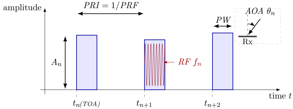
Figure 2.1. Parameters captured by a PDW for a short pulse train. Each pulse contributes a time of arrival (TOA) (the leading edge t_n on the time axis), a pulse width (PW), a peak amplitude A_n , and a carrier radio frequency (RF) f_n , shown as the fast oscillation inside the middle pulse. Successive pulses also define a PRI (equivalently a PRF = 1/PRI ). The inset shows the AOA \theta_n measured at the receive aperture relative to a boresight reference. A typical PDW stacks these per-pulse measurements into a vector \mathbf{x}_n = (f_n, PW_n, t_n, A_n, \theta_n) [1].
