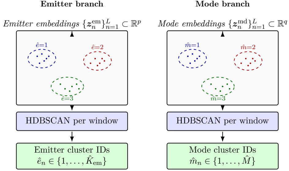
Figure 4.3. Inference-time decoding of branch embeddings into per-pulse cluster indices via Equation (4.14). Dots are pulse embeddings and dashed ellipses are HDBSCAN clusters in one window. The pipeline is identical on both branches and the integer outputs are local to each clustering instance; they acquire their interpretation from the supervision scope of Section 4.1, which differs between the two branches.
