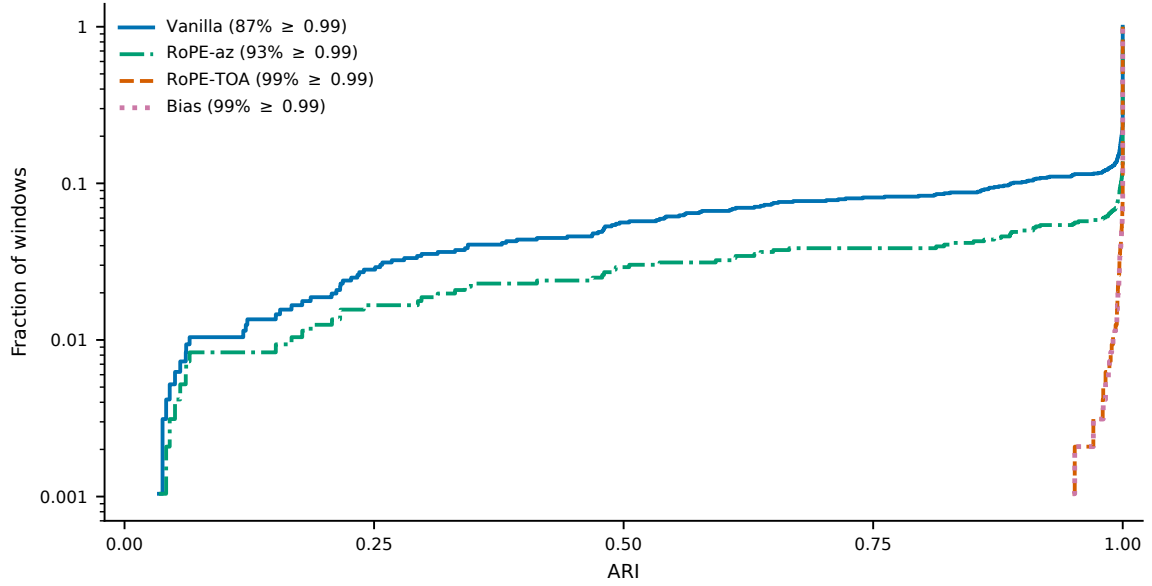
Figure 5.1. Empirical CDF of emitter ARI over the 960 non-overlapping test windows. The vertical axis is logarithmic.
